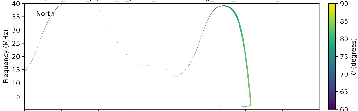
expres_earth_jupiter_io_jrm33_lossc-wid1deg_3kev_20130903_v11.cdf
