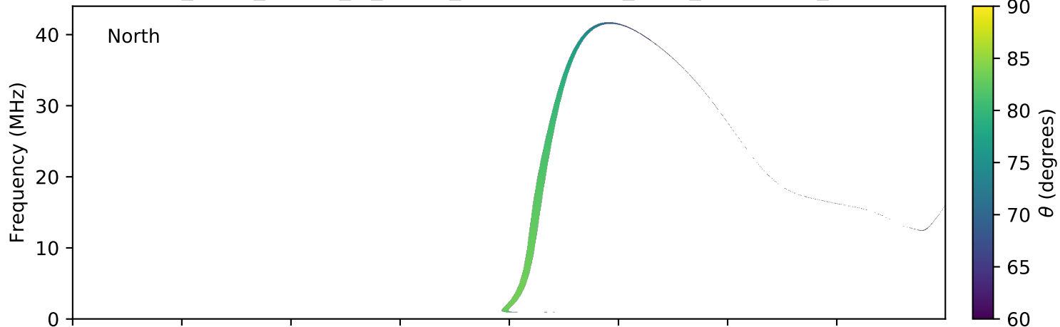
expres_earth_jupiter_io_jrm09_lossc-wid1deg_3kev_20130929_v01.cdf
