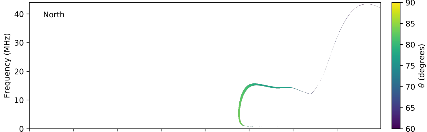
expres_earth_jupiter_io_jrm09_lossc-wid1deg_3kev_20130920_v01.cdf
