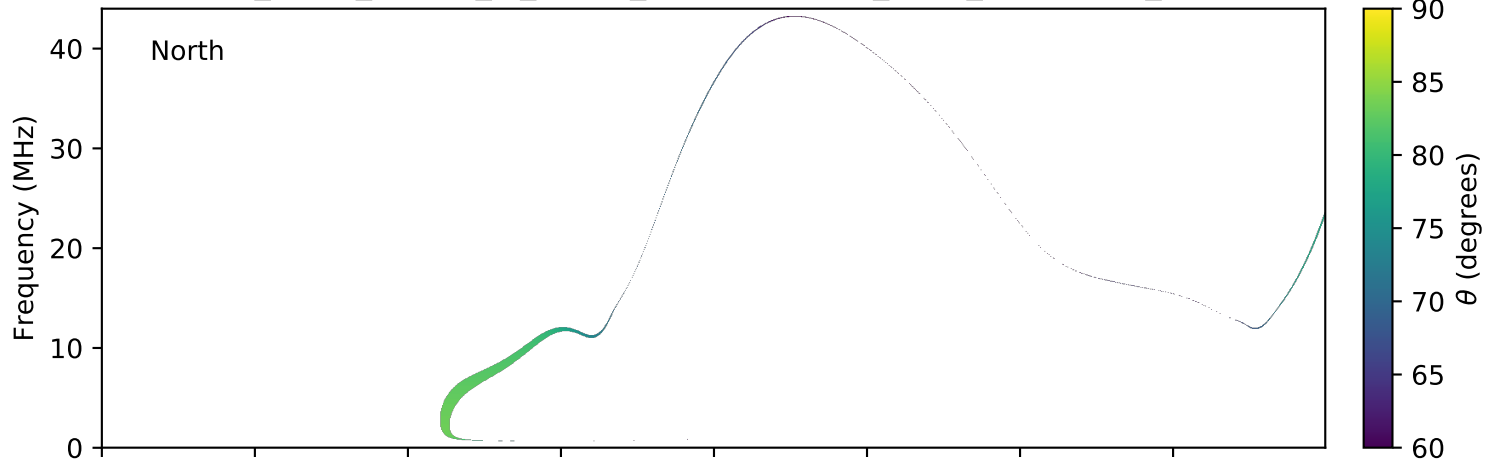
expres_earth_jupiter_io_jrm09_lossc-wid1deg_3kev_20130915_v01.cdf
