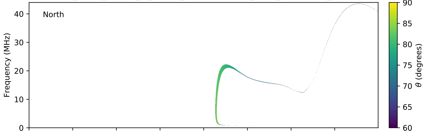
expres_earth_jupiter_io_jrm09_lossc-wid1deg_3kev_20130913_v01.cdf
