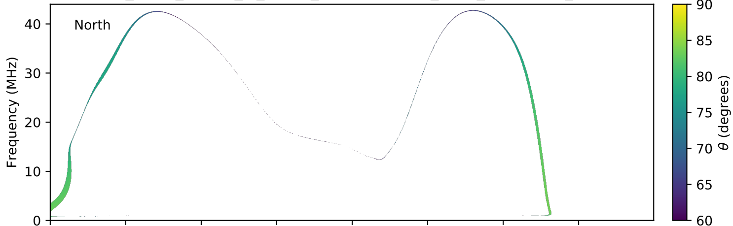
expres_earth_jupiter_io_jrm09_lossc-wid1deg_3kev_20130910_v01.cdf
