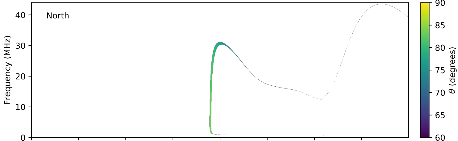
expres_earth_jupiter_io_jrm09_lossc-wid1deg_3kev_20130906_v01.cdf
