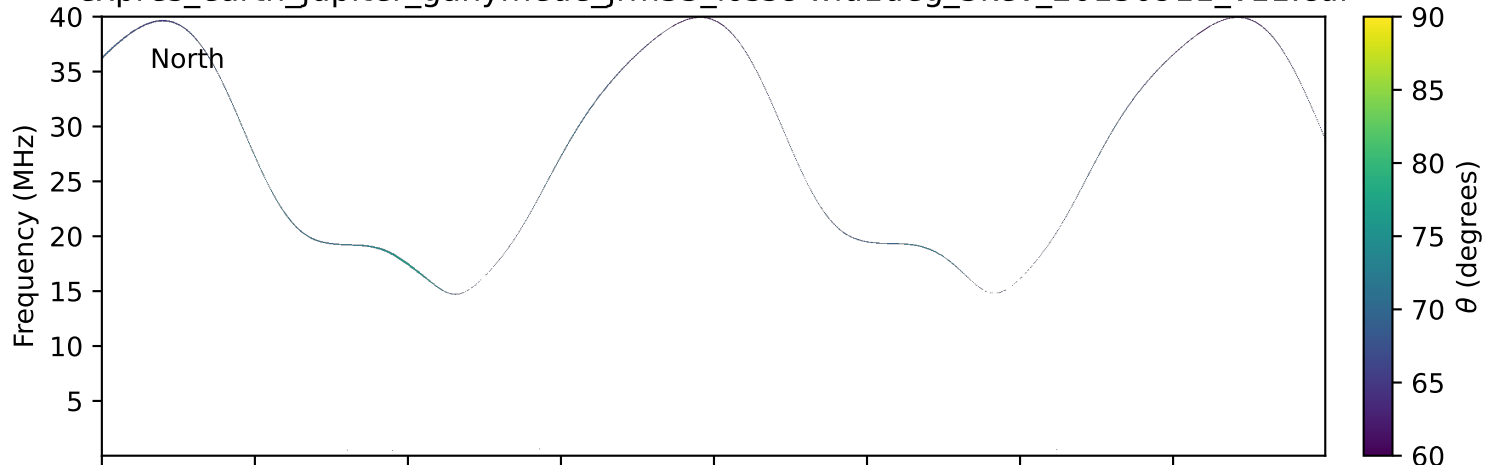
expres_earth_jupiter_ganymede_jrm33_lossc-wid1deg_3kev_20130911_v11.cdf
