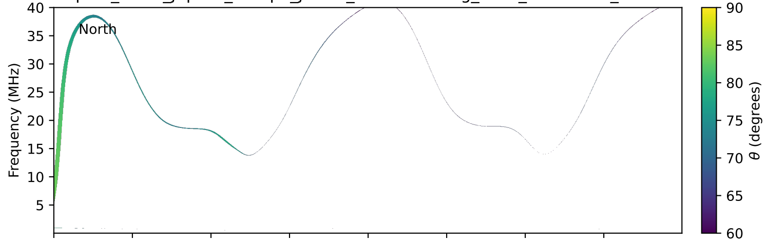
expres_earth_jupiter_europa_jrm33_lossc-wid1deg_3kev_20130906_v11.cdf
