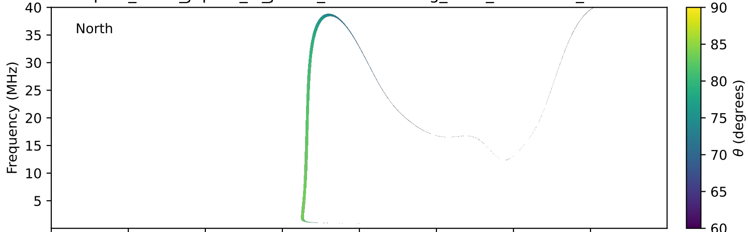
expres_earth_jupiter_io_jrm33_lossc-wid1deg_3kev_20130830_v11.cdf
