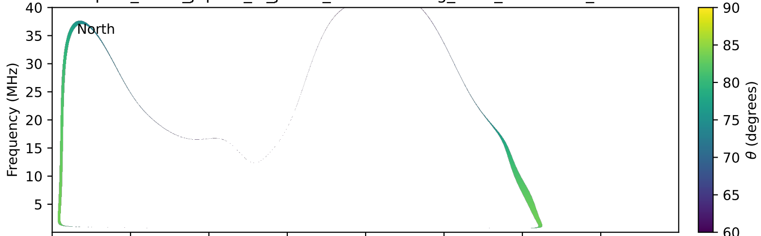
expres_earth_jupiter_io_jrm33_lossc-wid1deg_3kev_20130818_v11.cdf
