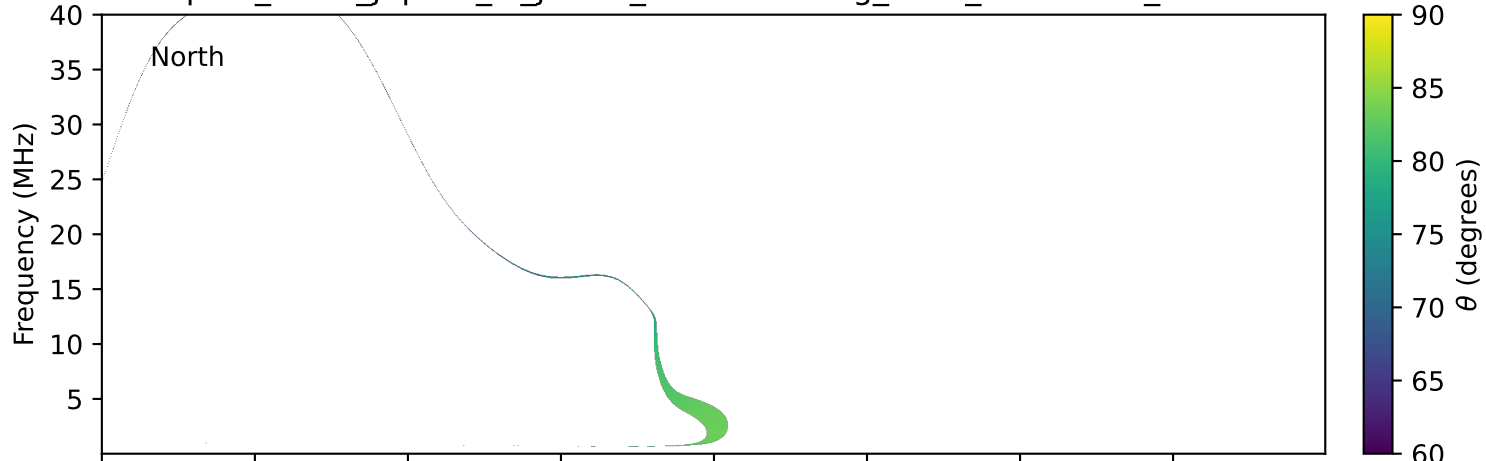
expres_earth_jupiter_io_jrm33_lossc-wid1deg_3kev_20130813_v11.cdf
