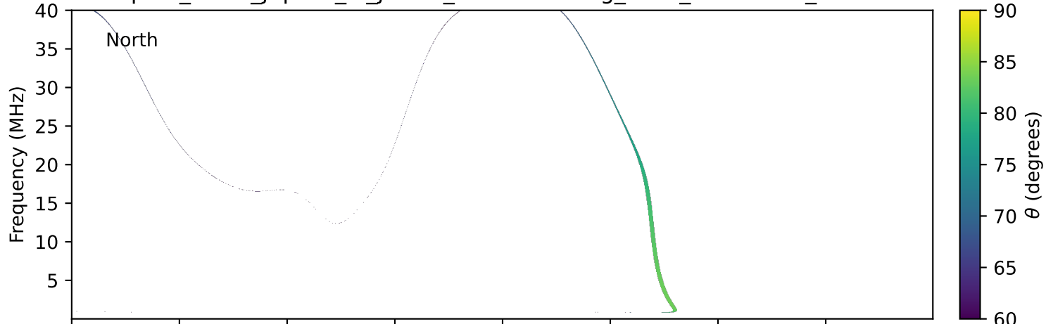
expres_earth_jupiter_io_jrm33_lossc-wid1deg_3kev_20130811_v11.cdf
