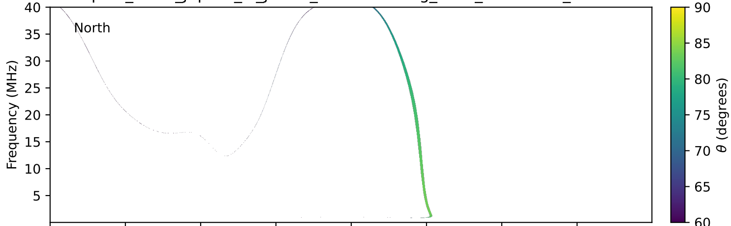
expres_earth_jupiter_io_jrm33_lossc-wid1deg_3kev_20130804_v11.cdf
