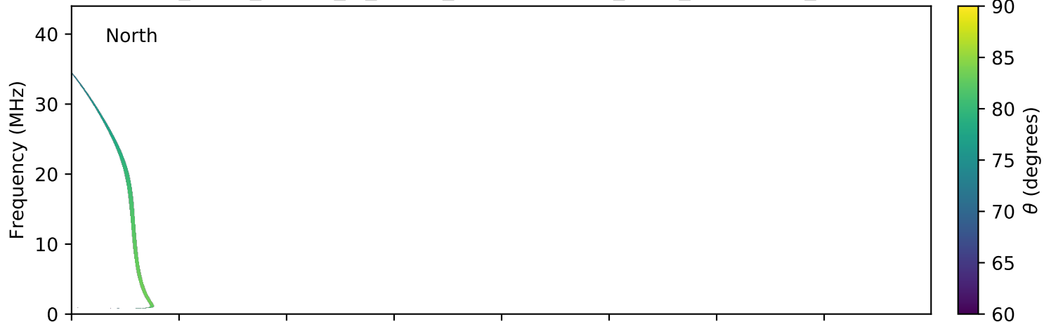
expres_earth_jupiter_io_jrm09_lossc-wid1deg_3kev_20130824_v01.cdf
