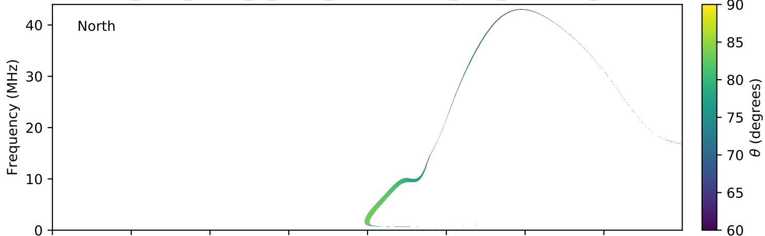
expres_earth_jupiter_io_jrm09_lossc-wid1deg_3kev_20130821_v01.cdf
