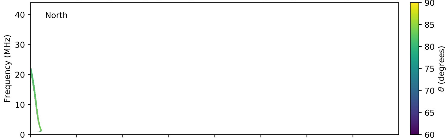
expres_earth_jupiter_io_jrm09_lossc-wid1deg_3kev_20130817_v01.cdf
