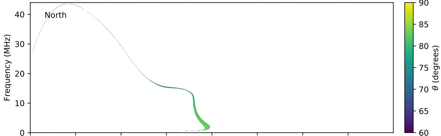
expres_earth_jupiter_io_jrm09_lossc-wid1deg_3kev_20130813_v01.cdf
