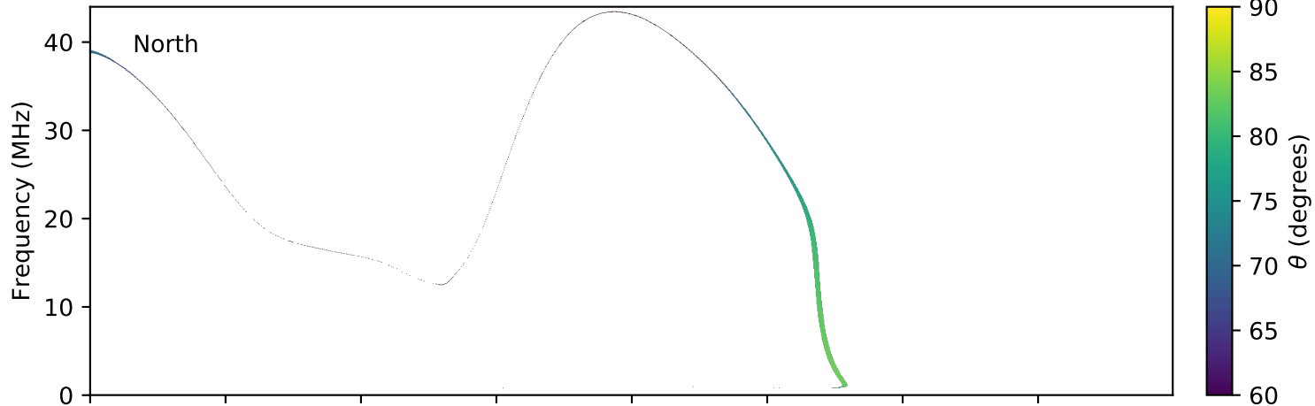
expres_earth_jupiter_io_jrm09_lossc-wid1deg_3kev_20130811_v01.cdf
