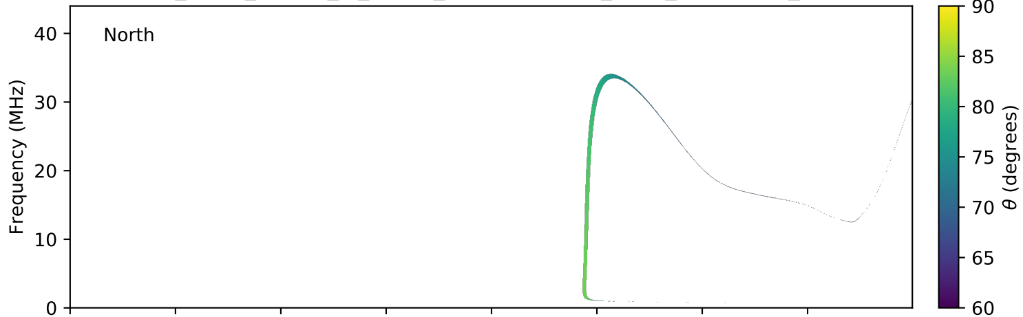
expres_earth_jupiter_io_jrm09_lossc-wid1deg_3kev_20130805_v01.cdf
