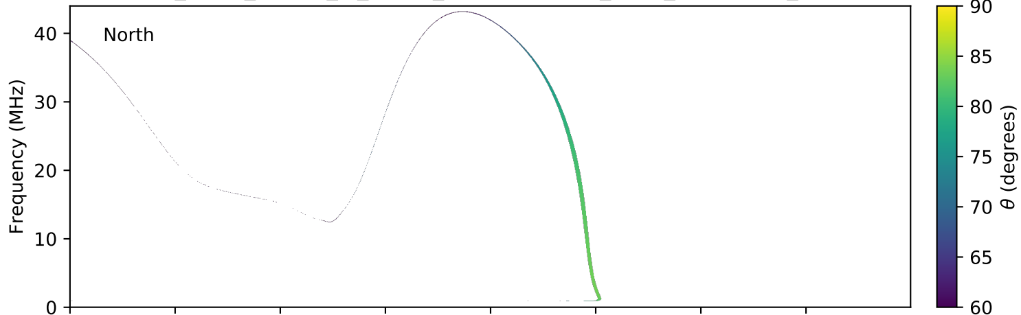
expres_earth_jupiter_io_jrm09_lossc-wid1deg_3kev_20130804_v01.cdf
