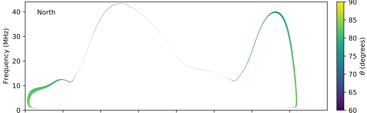
expres_earth_jupiter_io_jrm09_lossc-wid1deg_3kev_20130802_v01.cdf
