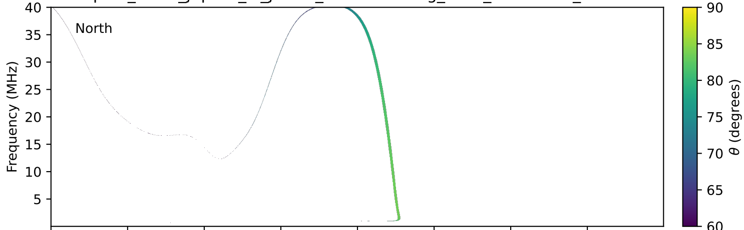
expres_earth_jupiter_io_jrm33_lossc-wid1deg_3kev_20130728_v11.cdf
