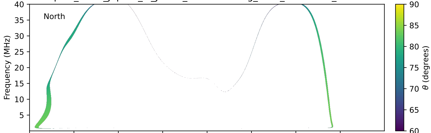
expres_earth_jupiter_io_jrm33_lossc-wid1deg_3kev_20130724_v11.cdf
