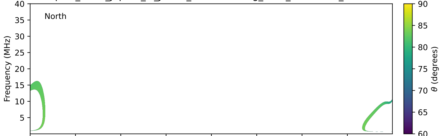
expres_earth_jupiter_io_jrm33_lossc-wid1deg_3kev_20130716_v11.cdf
