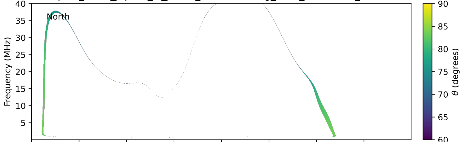
expres_earth_jupiter_io_jrm33_lossc-wid1deg_3kev_20130701_v11.cdf
