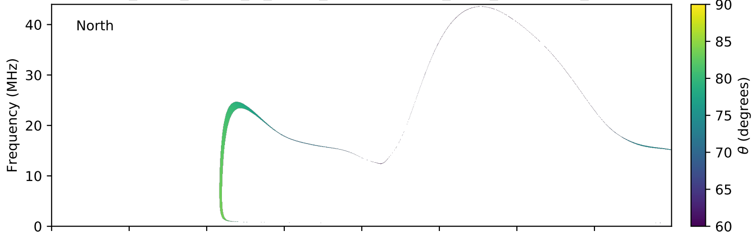
expres_earth_jupiter_io_jrm09_lossc-wid1deg_3kev_20130731_v01.cdf
