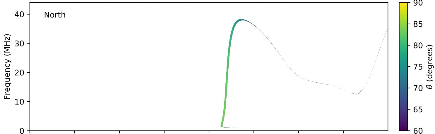
expres_earth_jupiter_io_jrm09_lossc-wid1deg_3kev_20130729_v01.cdf
