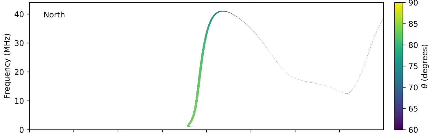
expres_earth_jupiter_io_jrm09_lossc-wid1deg_3kev_20130722_v01.cdf
