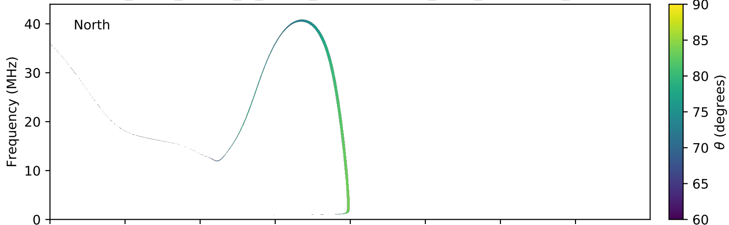
expres_earth_jupiter_io_jrm09_lossc-wid1deg_3kev_20130721_v01.cdf
