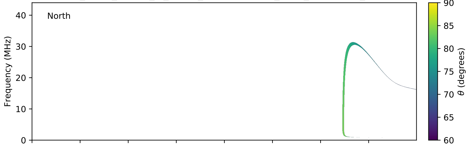
expres_earth_jupiter_io_jrm09_lossc-wid1deg_3kev_20130711_v01.cdf
