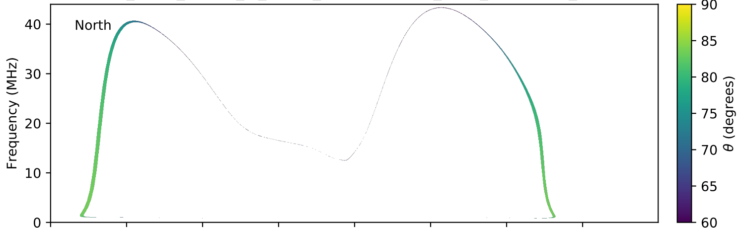
expres_earth_jupiter_io_jrm09_lossc-wid1deg_3kev_20130710_v01.cdf
