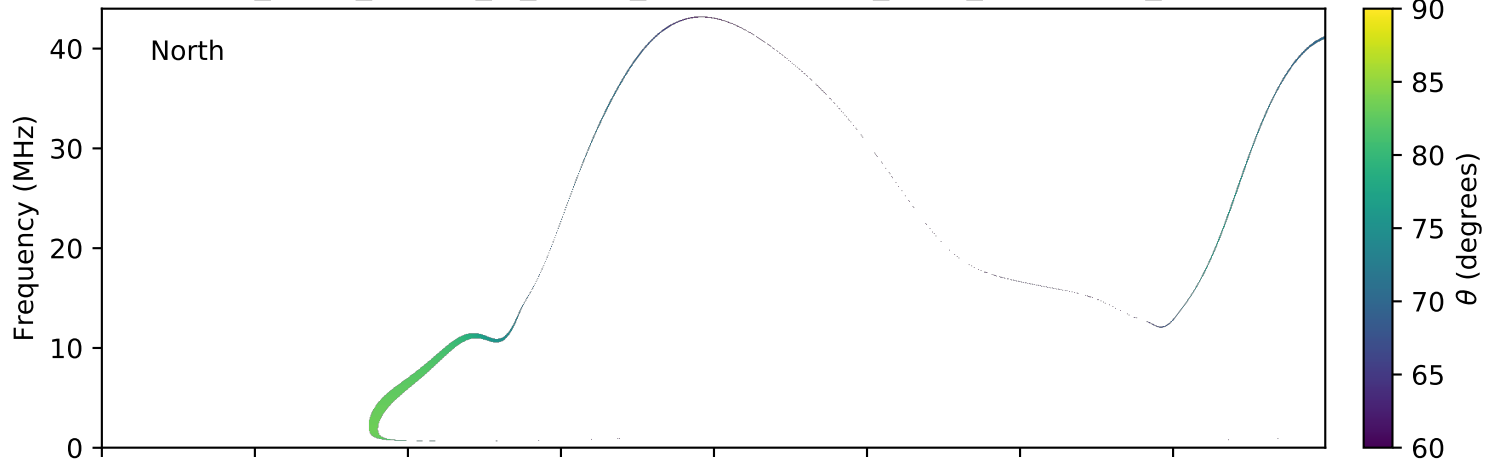
expres_earth_jupiter_io_jrm09_lossc-wid1deg_3kev_20130708_v01.cdf
