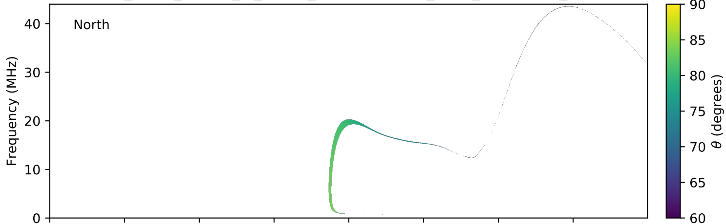
expres_earth_jupiter_io_jrm09_lossc-wid1deg_3kev_20130706_v01.cdf
