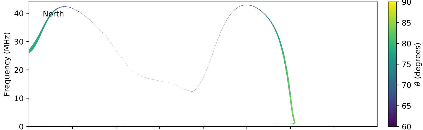
expres_earth_jupiter_io_jrm09_lossc-wid1deg_3kev_20130703_v01.cdf
