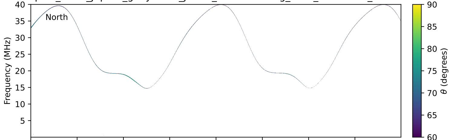
expres_earth_jupiter_ganymede_jrm33_lossc-wid1deg_3kev_20130713_v11.cdf
