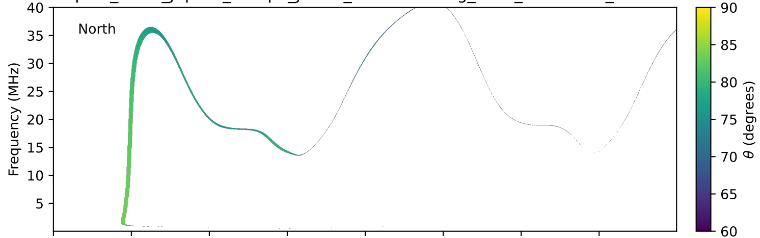
expres_earth_jupiter_europa_jrm33_lossc-wid1deg_3kev_20130710_v11.cdf
