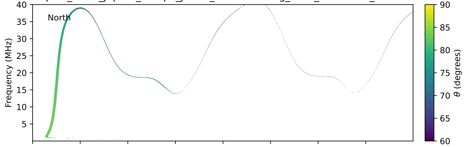
expres_earth_jupiter_europa_jrm33_lossc-wid1deg_3kev_20130703_v11.cdf
