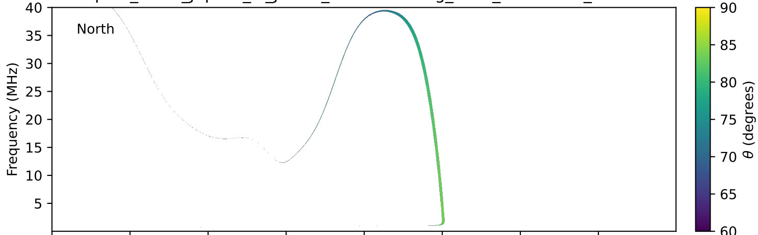
expres_earth_jupiter_io_jrm33_lossc-wid1deg_3kev_20130624_v11.cdf
