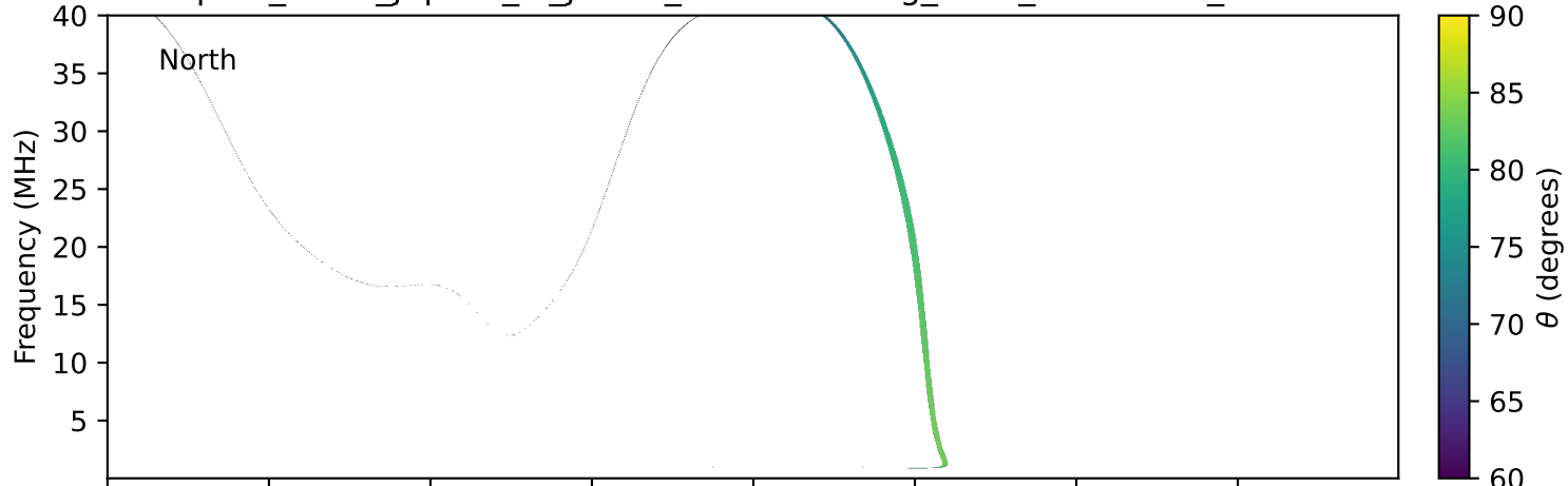
expres_earth_jupiter_io_jrm33_lossc-wid1deg_3kev_20130617_v11.cdf
