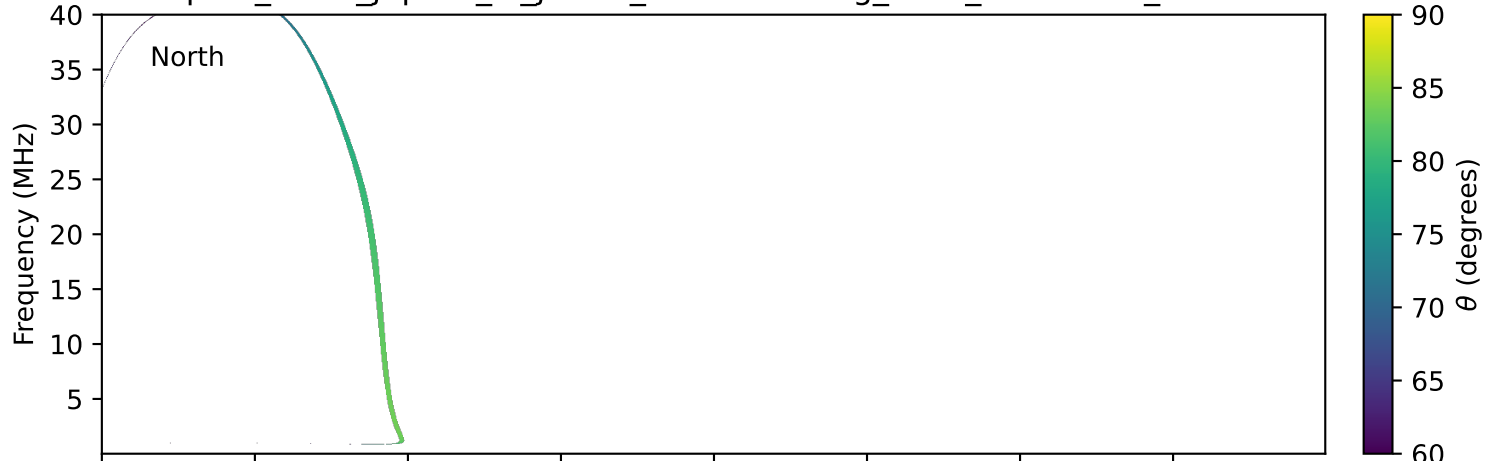
expres_earth_jupiter_io_jrm33_lossc-wid1deg_3kev_20130605_v11.cdf
