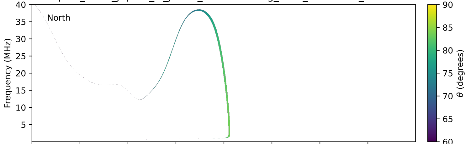
expres_earth_jupiter_io_jrm33_lossc-wid1deg_3kev_20130603_v11.cdf
