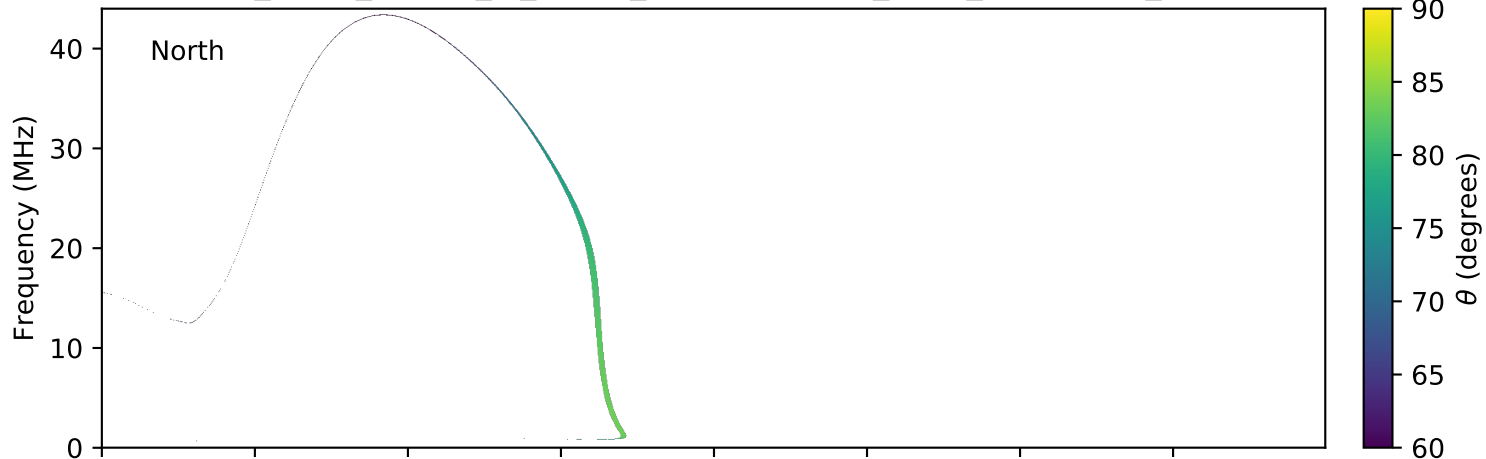
expres_earth_jupiter_io_jrm09_lossc-wid1deg_3kev_20130628_v01.cdf
