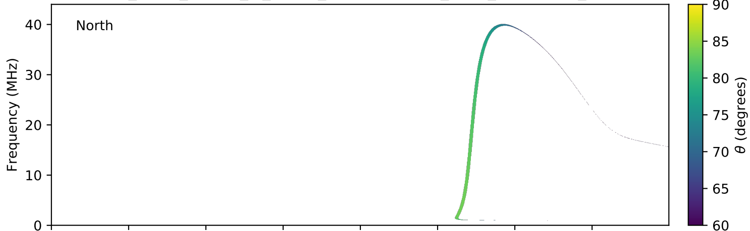
expres_earth_jupiter_io_jrm09_lossc-wid1deg_3kev_20130627_v01.cdf
