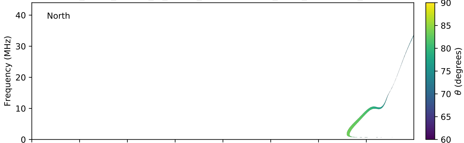
expres_earth_jupiter_io_jrm09_lossc-wid1deg_3kev_20130625_v01.cdf
