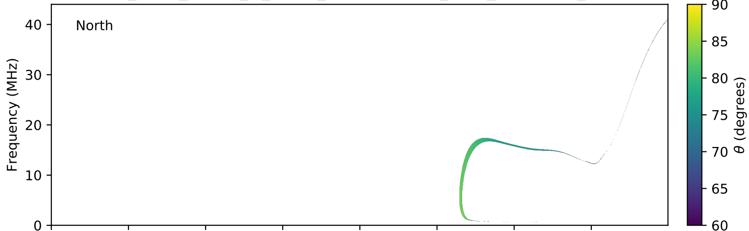
expres_earth_jupiter_io_jrm09_lossc-wid1deg_3kev_20130611_v01.cdf
