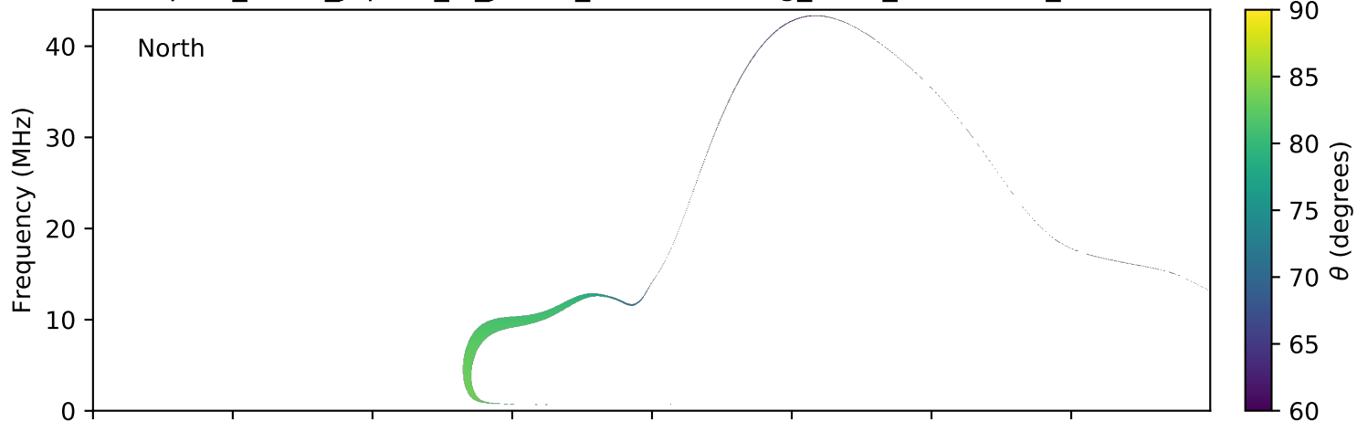
expres_earth_jupiter_io_jrm09_lossc-wid1deg_3kev_20130606_v01.cdf
