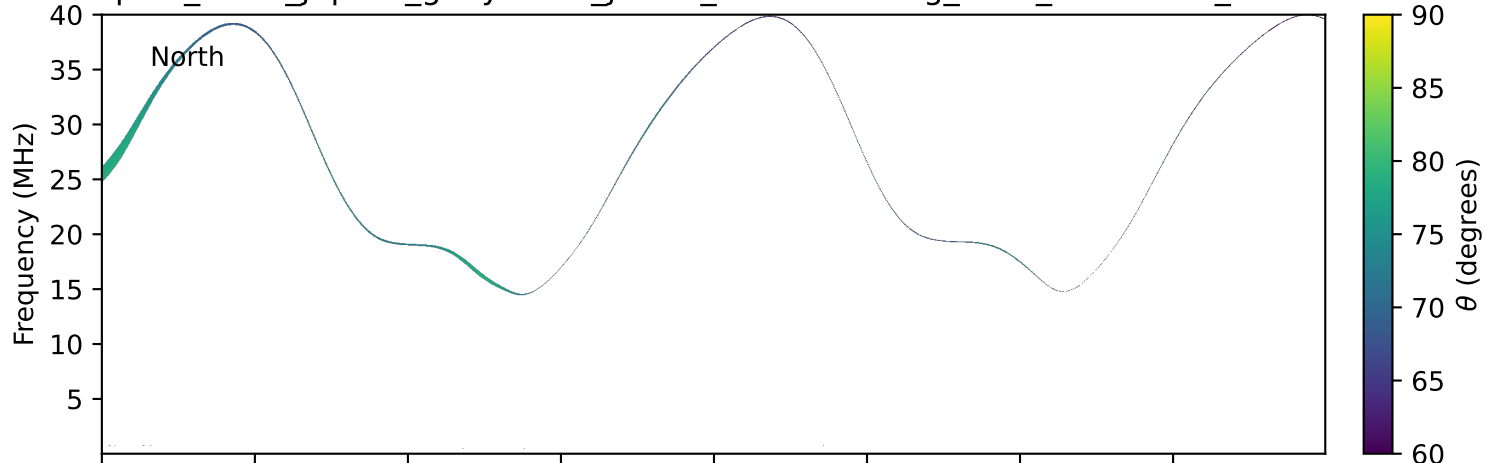
expres_earth_jupiter_ganymede_jrm33_lossc-wid1deg_3kev_20130614_v11.cdf
