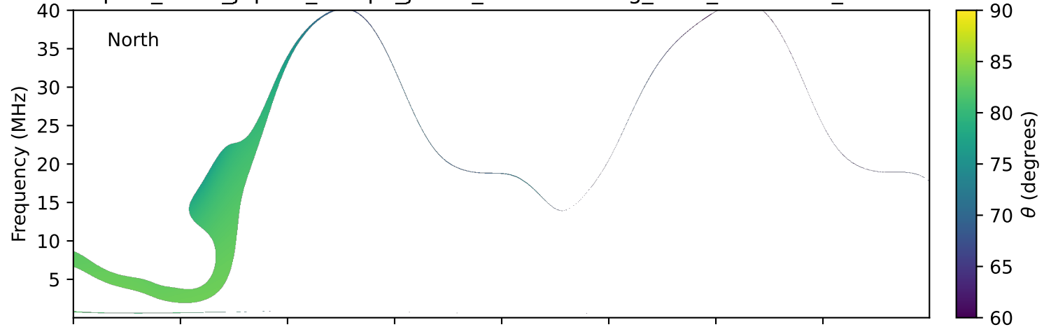
expres_earth_jupiter_europa_jrm33_lossc-wid1deg_3kev_20130608_v11.cdf
