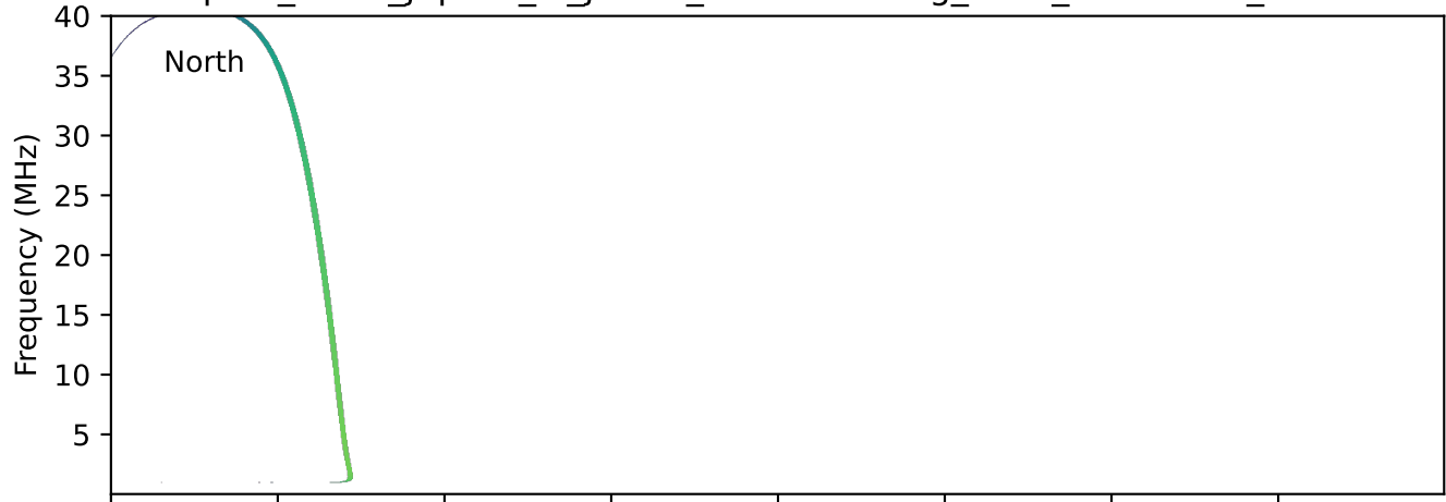
expres_earth_jupiter_io_jrm33_lossc-wid1deg_3kev_20130529_v11.cdf
